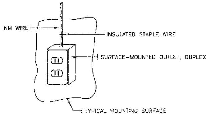
TYPICAL CONVENIENCE OUTLET INSTALLATION
