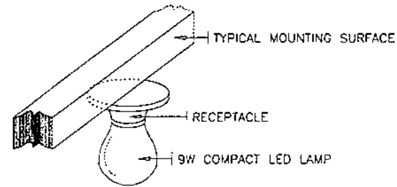
TYPICAL LIGHTING FIXTURE INSTALLATION
