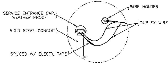
DETAIL "B"
